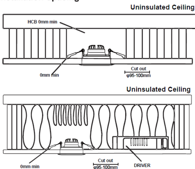
Fig 1: Installation Spacing
